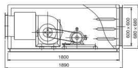
YDF-A-No2.8外形尺寸
