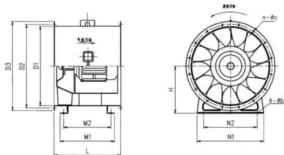
HTF-III型轴流式消防排烟风机外形及安装尺寸
